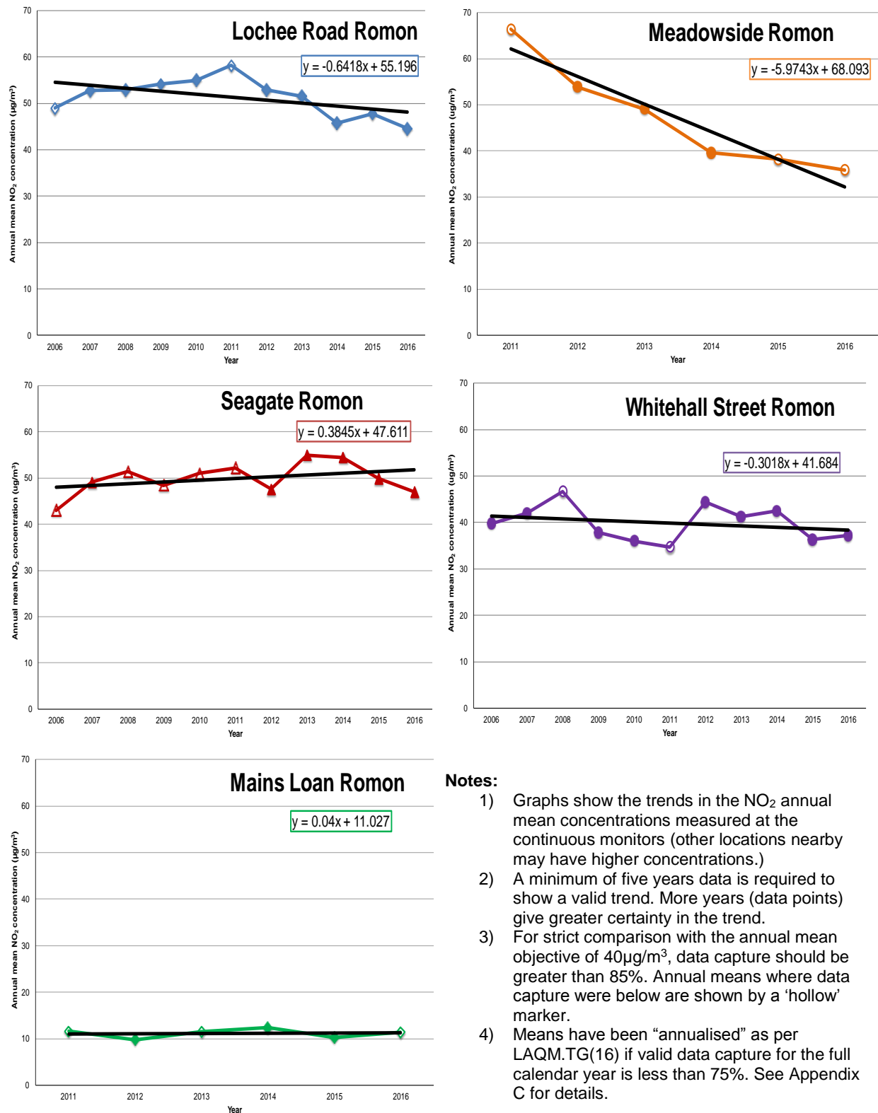
Figure A.3a Trends in NO 2 at Automatic monitors
