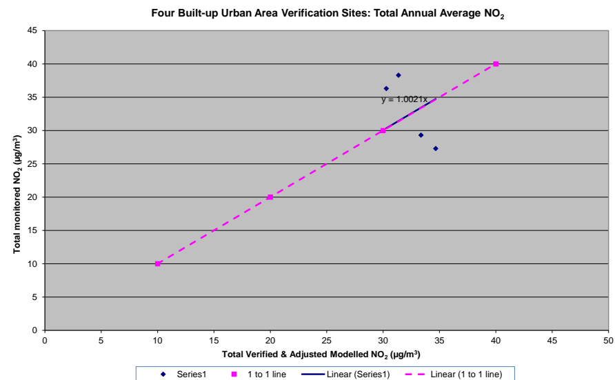
Graph of Monitored vs Modelled NO 2 Results after Adjustment
