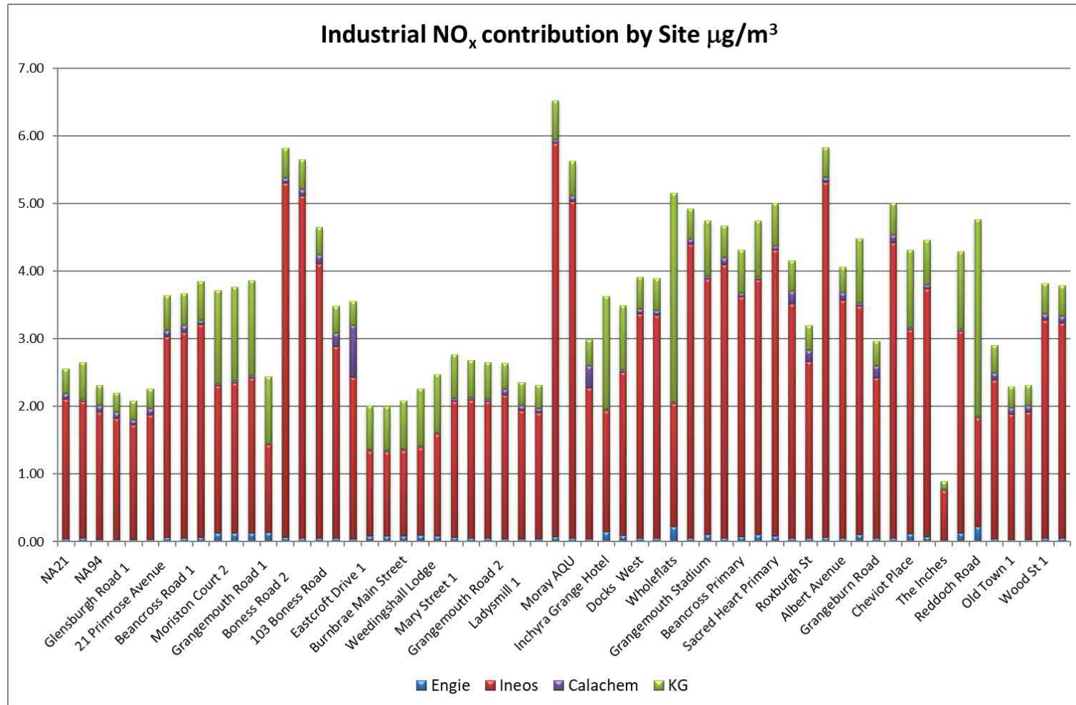
Chart 10-5 NO x contribution contribution by industrial operator
