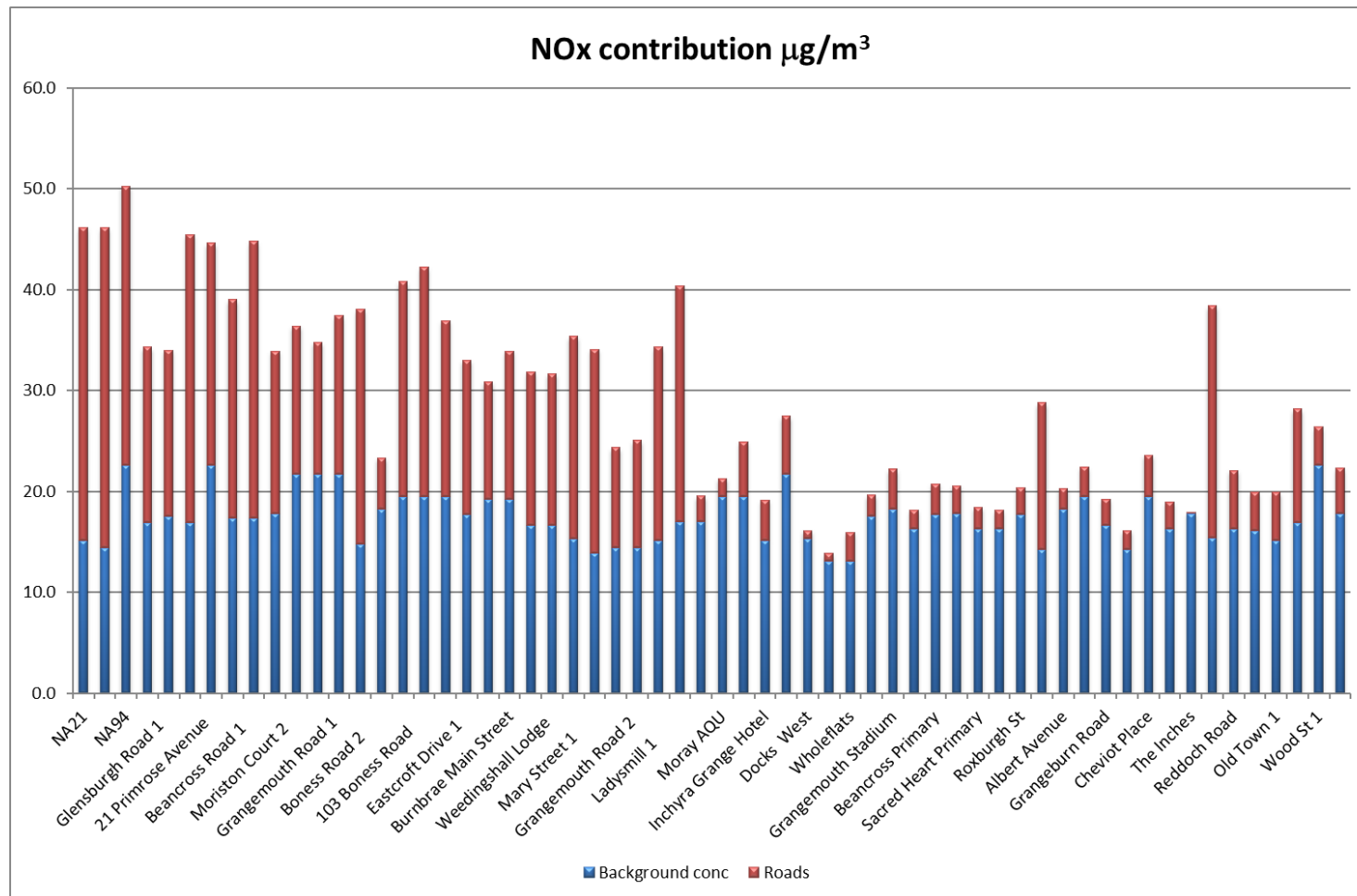
Chart 10-1 NOx contribution by location
