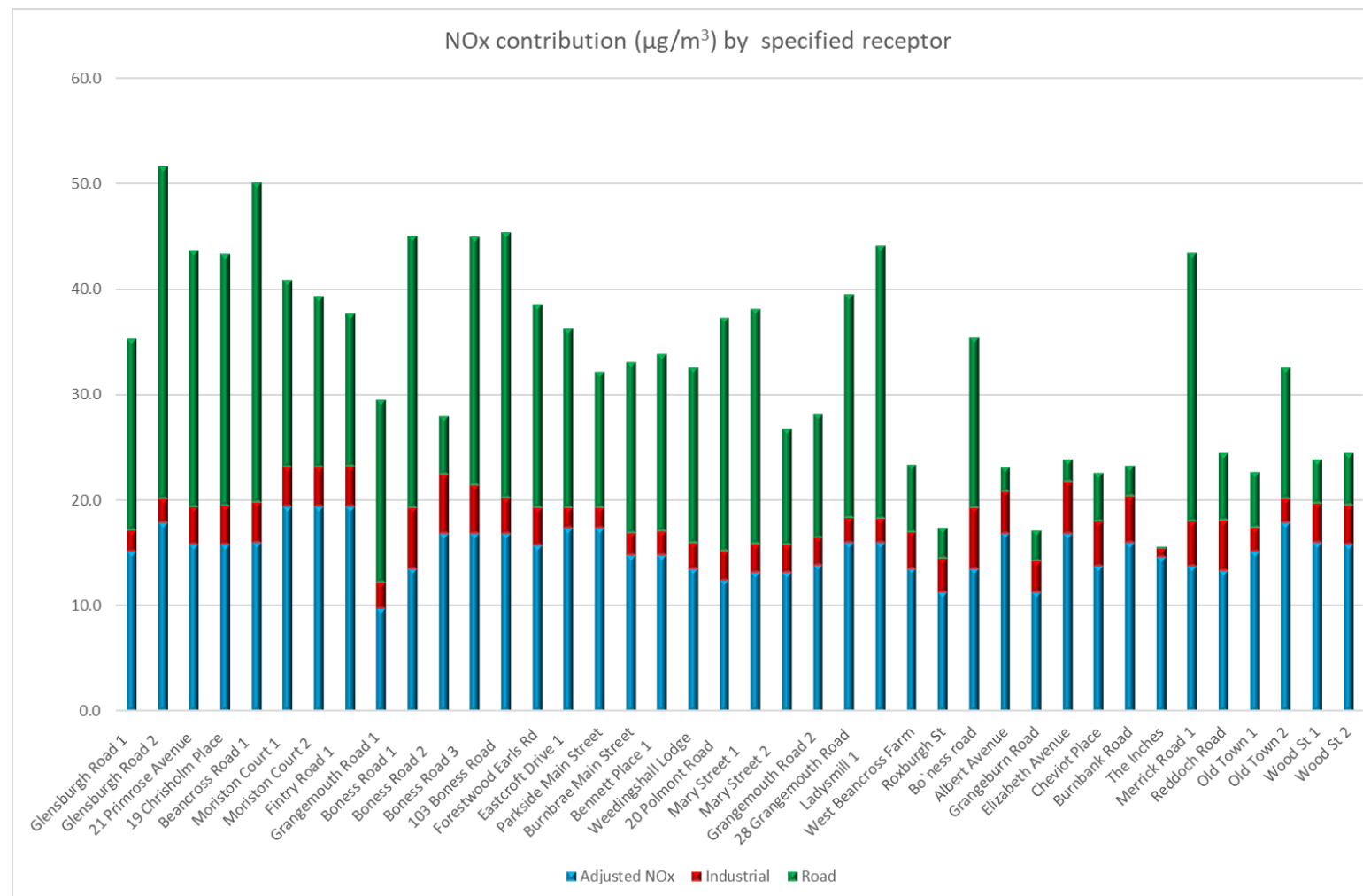
Chart 10-6 NOx ( \mu\text{g}/\text{m}^3 ) contribution by source for each receptor
