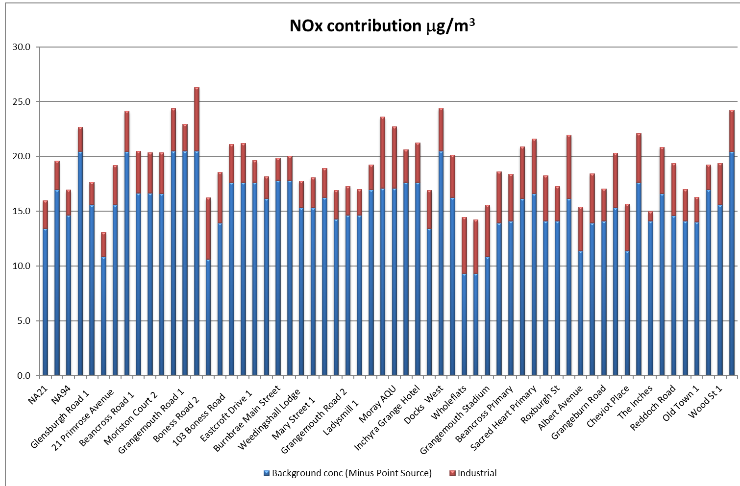
Chart 10-4 NOx contribution by location from industrial emissions
