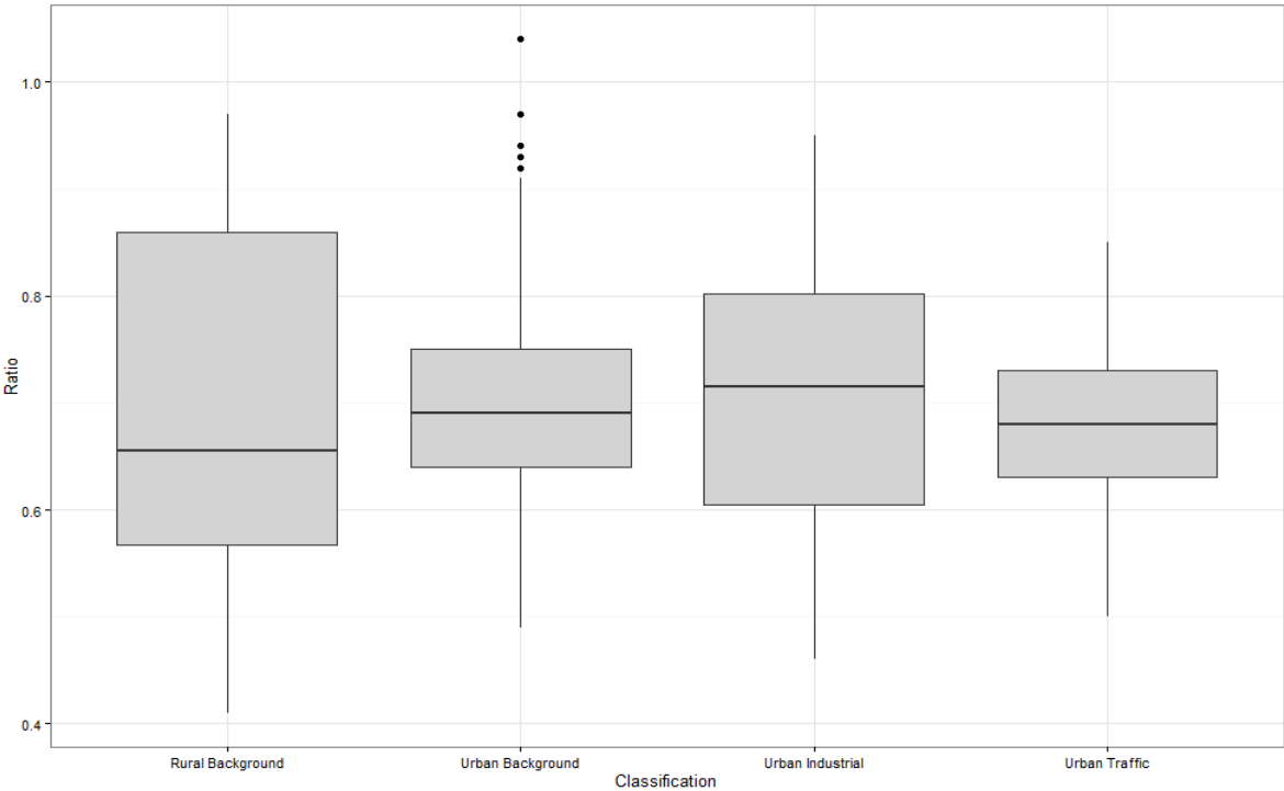
Figure B.6 – A Box and Whisker Plot showing the Spread in the Annual Average Ratio of \text{PM}_{2.5}/\text{PM}_{10} as a Function of Site Classification for All Years
