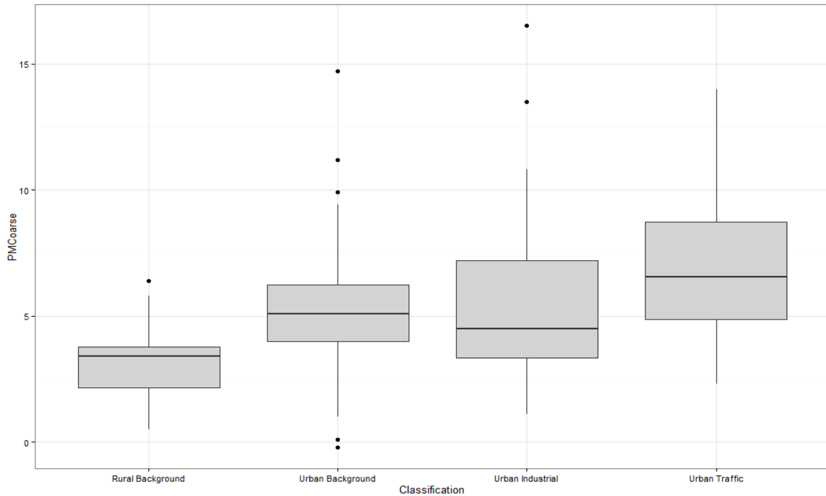
Figure B.4 – A Box and Whisker Plot showing the Spread in the Annual Average \text{PM}_{\text{Coarse}} \mu\text{g}/\text{m}^3 as a Function of Site Classification for All Years
