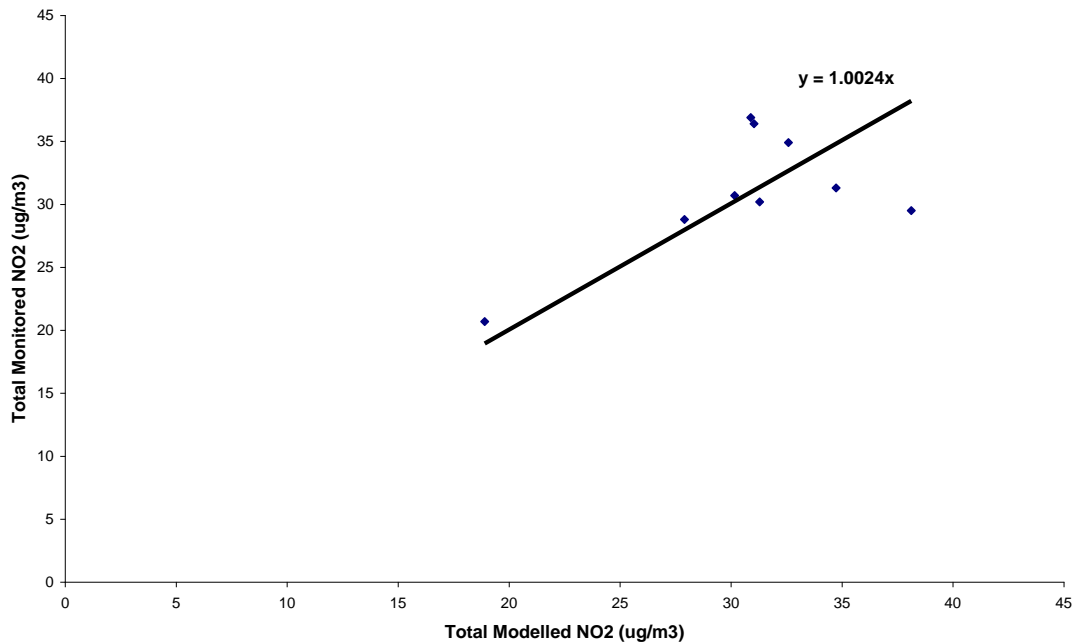
Figure 3.1: Modelled vs monitored annual average NO 2
