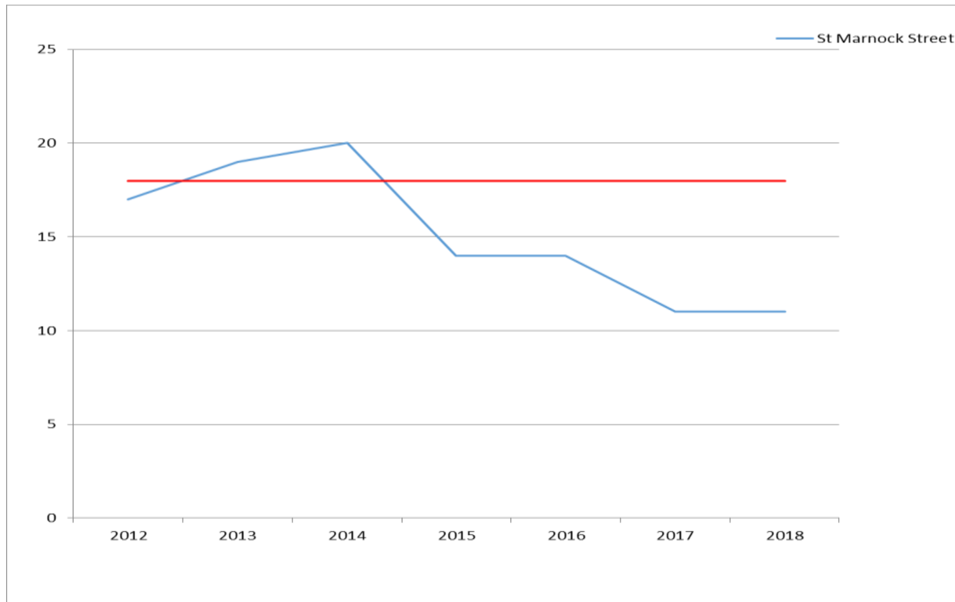
Figure A.6 Trends in Annual Mean PM 10 Concentrations Measured at St. Marnock Street Automatic
