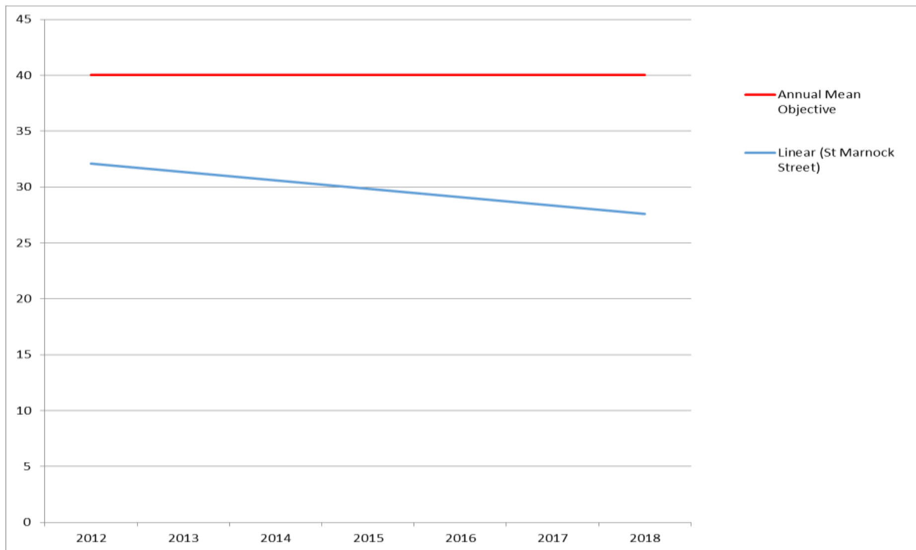
Figure A.2 Trends in Annual Mean Nitrogen Dioxide Concentrations Measured at St. Marnock Street Automatic Monitor – Linear
