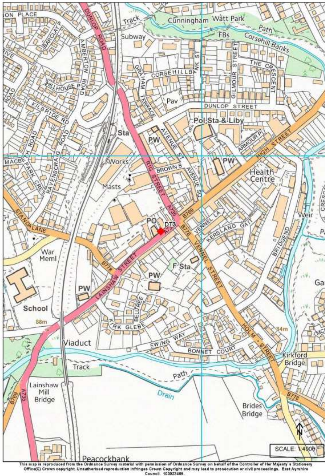
Figure G.7: Stewarton NO2 Diffusion Tube Locations
