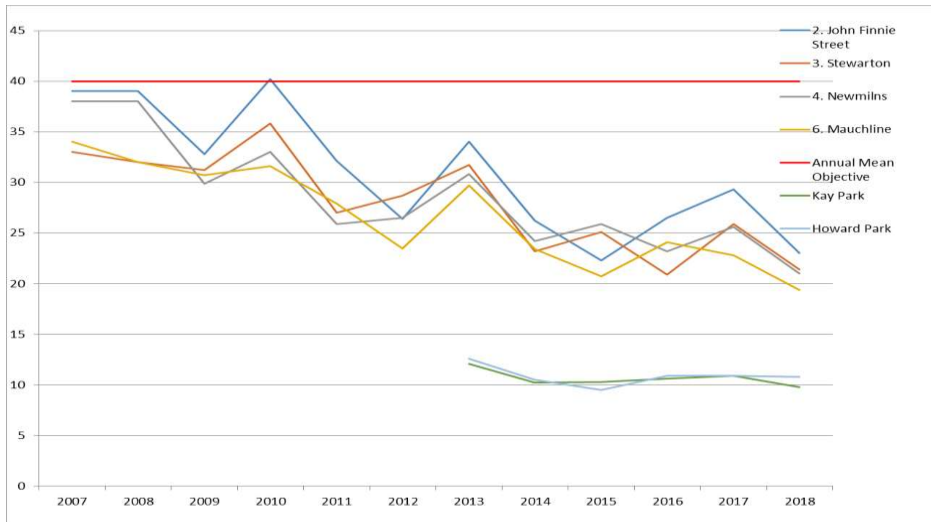
Figure A.3 Trends in Annual Mean Nitrogen Dioxide Concentrations Measured at Long Term Diffusion Tube Monitoring Sites 2007-2018
