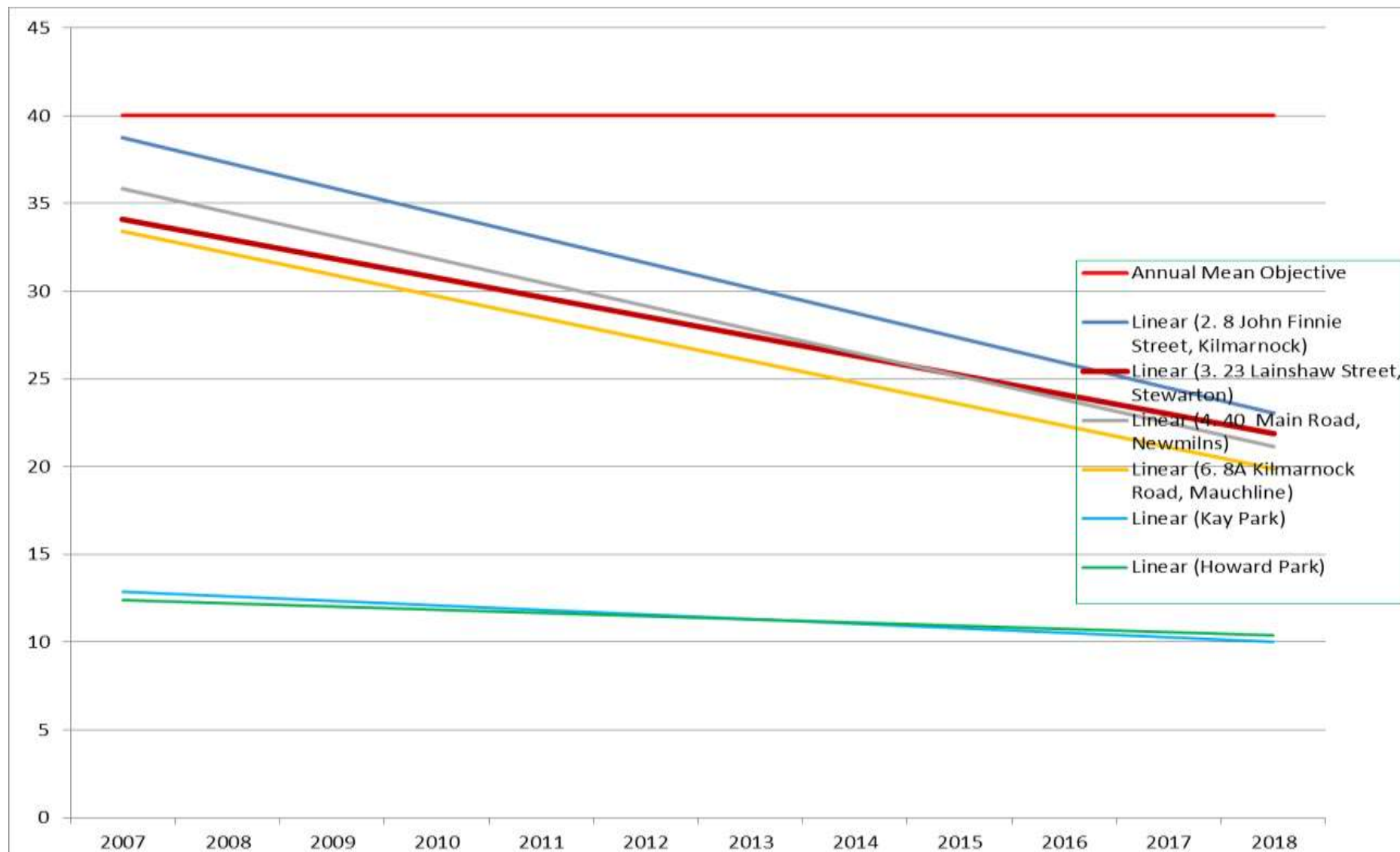
Figure A.4 Trends in Annual Mean Nitrogen Dioxide Concentrations Measured at Long Term Diffusion Tube Monitoring Sites - Linear 2007-2018
