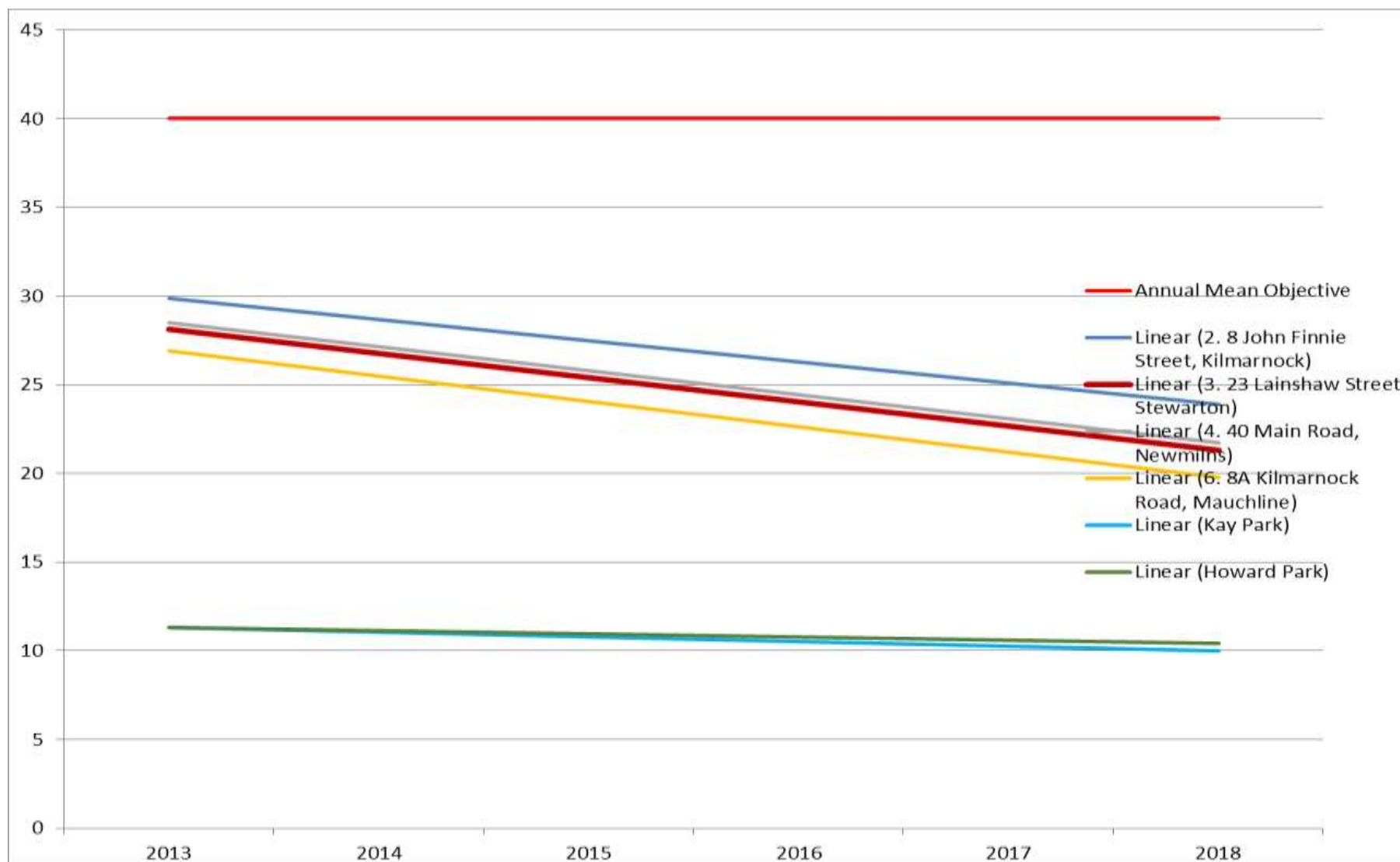
Figure A.5 Trends in Annual Mean Nitrogen Dioxide Concentrations Measured at Long Term Diffusion Tube Monitoring Sites – Linear 2013 – 2018
