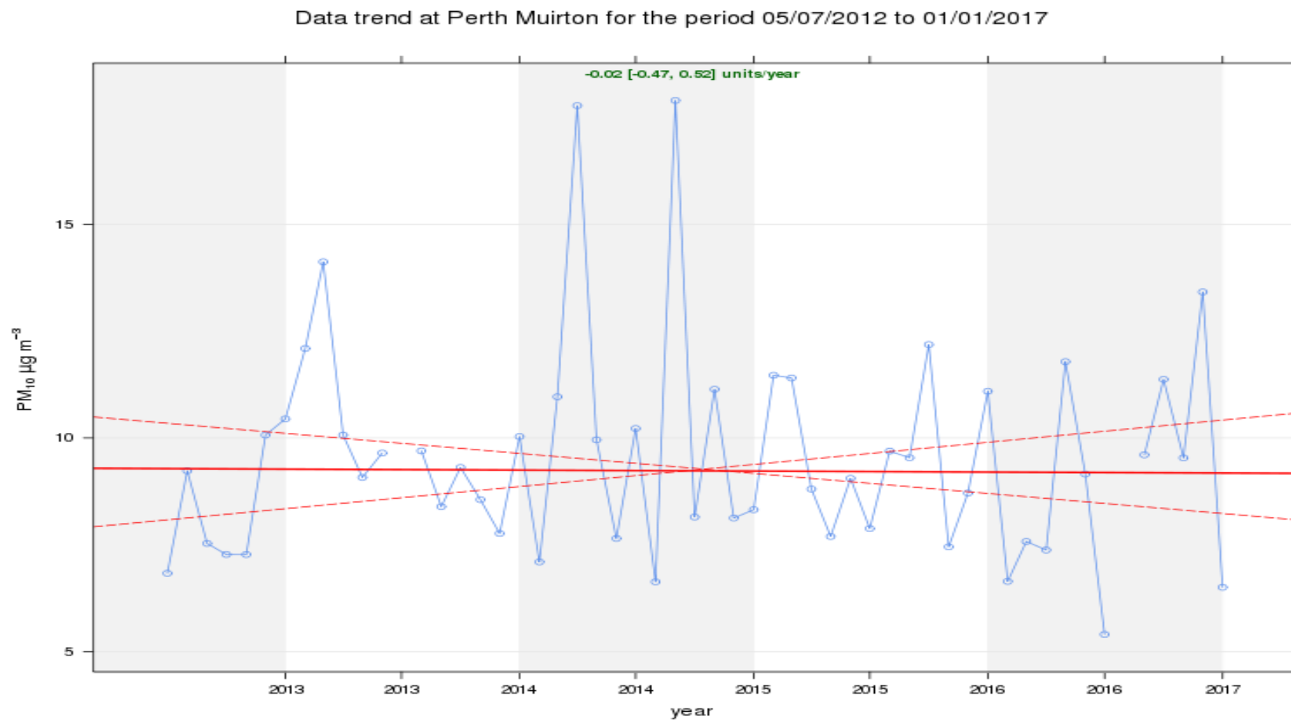
Figure 7 Annual Mean Trend for PM 10 at Muirton
