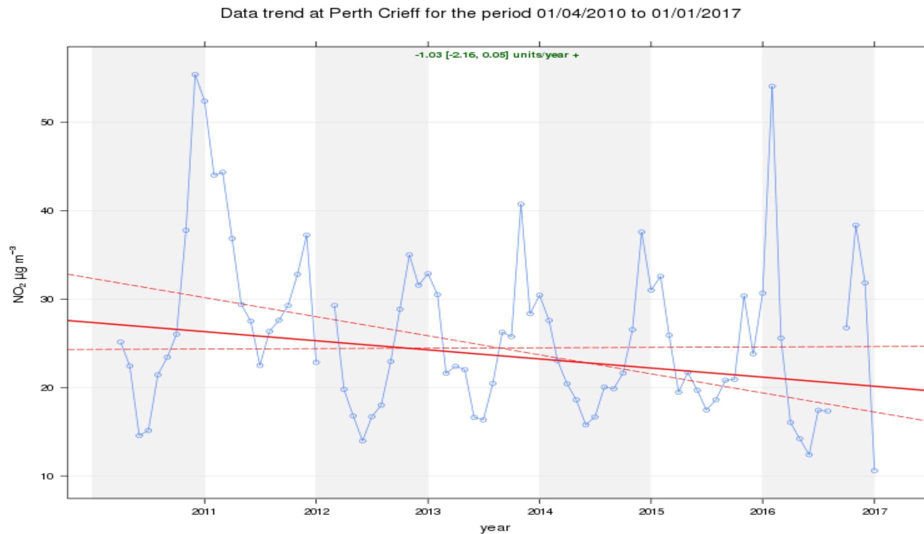
Figure 3 Annual Mean Trend for NO 2 at Crieff
