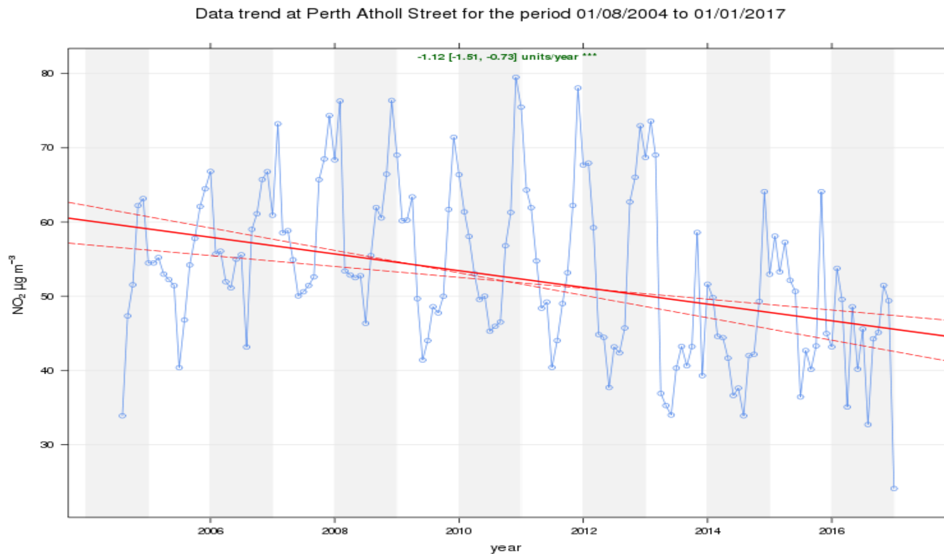
Figure 2 Annual Mean Trend for NO 2 at Atholl St
