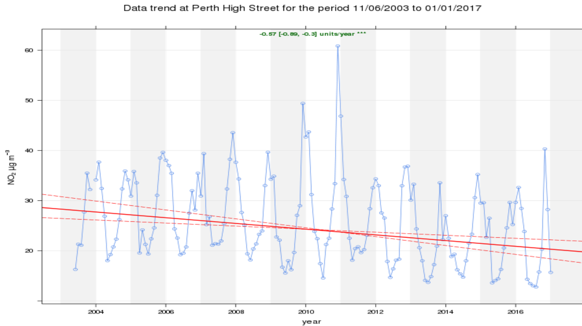
Figure 1 Annual Mean Trend for NO 2 at High St
