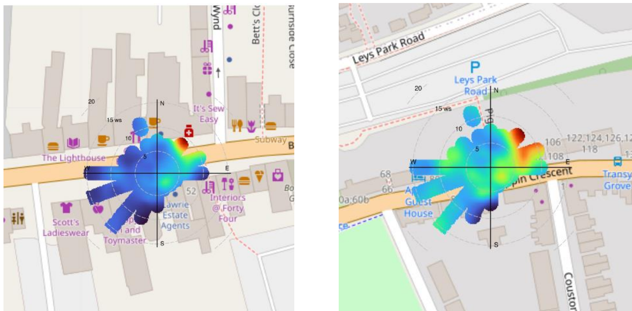
Figure 3-16 Polar plots of PM 10 concentrations by wind speed and direction
