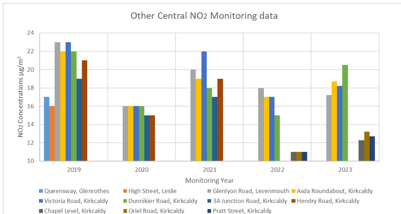
Figure A-7 Other Central Diffusion Tube Annual Mean Concentrations 2019-2023 ( \mu\text{g m}^{-3} )
