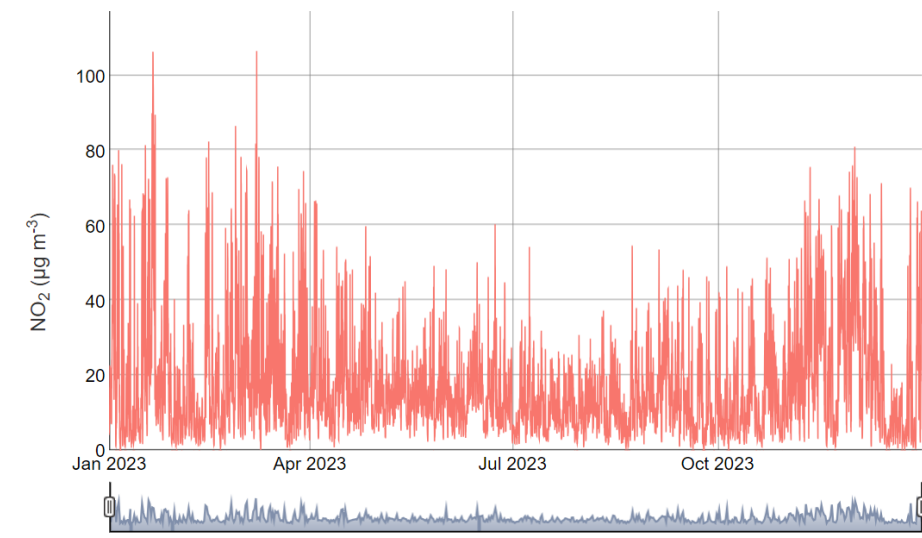
Figure F-4 Rosyth NO 2 time series
