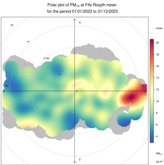
Figure F-32 Rosyth PM 10 polar plot
