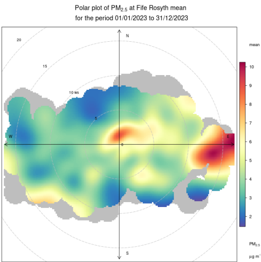
Figure F-36 Rosyth PM 2.5 polar plot
