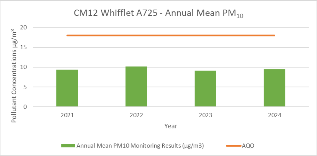
Figure A8 : Annual Mean Concentrations of PM 10 ay CM12 Whifflet A725
