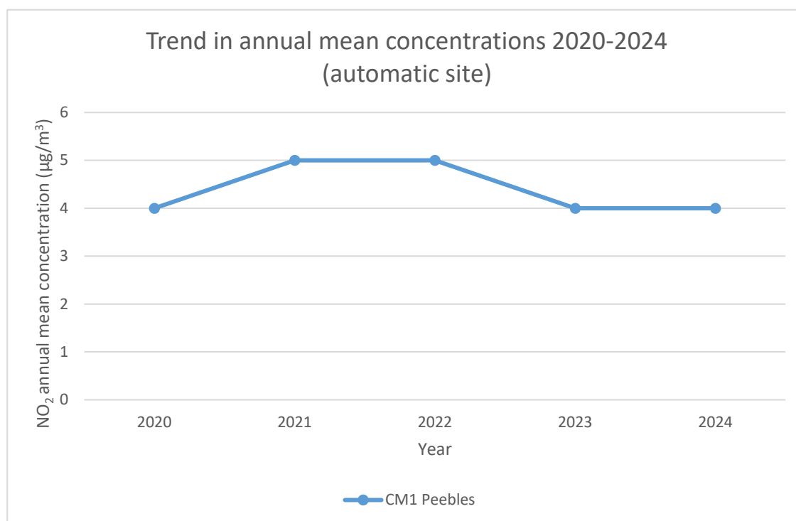
Figure A.1 - Trend in measured annual mean 2020-2024 (automatic site)
